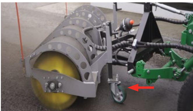
Support wheels
